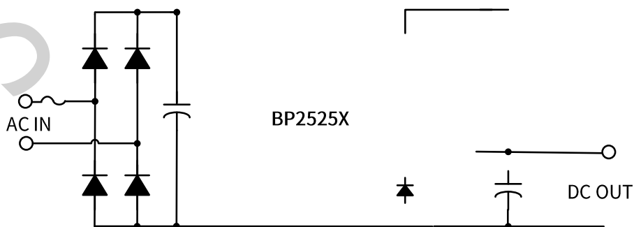
Figure 1. Typical application circuit for BP2525X
